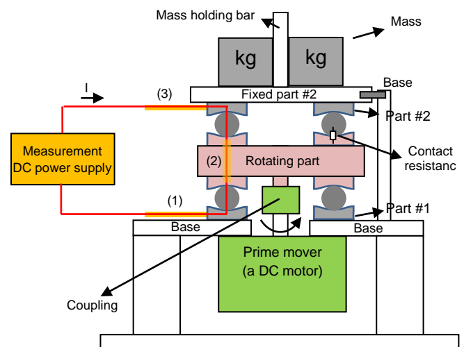
Fig. 1. Axial bearing test setup to measure the contact resistance between the ball and the ring
