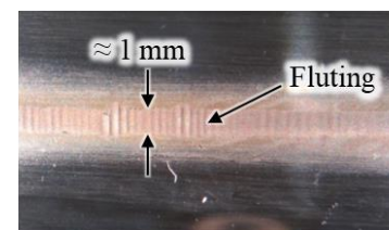
Fig. 2. Bearing surface damage (fluting), Rotor-to-earth bearing current, Apparent current density 1 \text{ A/mm}^2 , After 1000 hours operation
