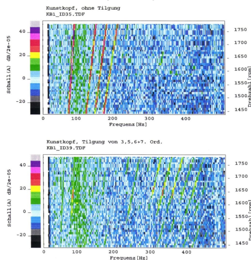
Campbell-Diagramme
