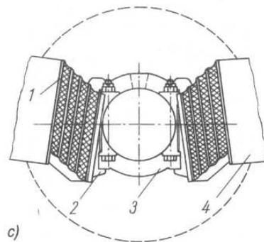
Chevron-Feder
